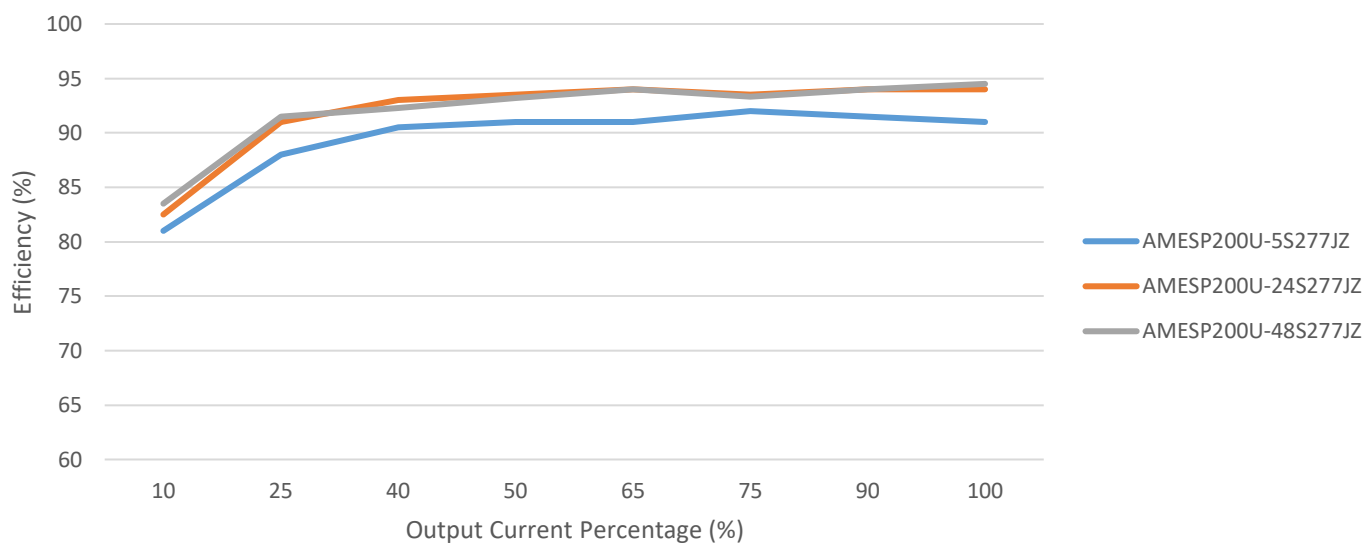
Efficiency vs Output Load (Vin=230VAC)
