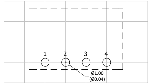
Grid size: 2.54*2.54mm
