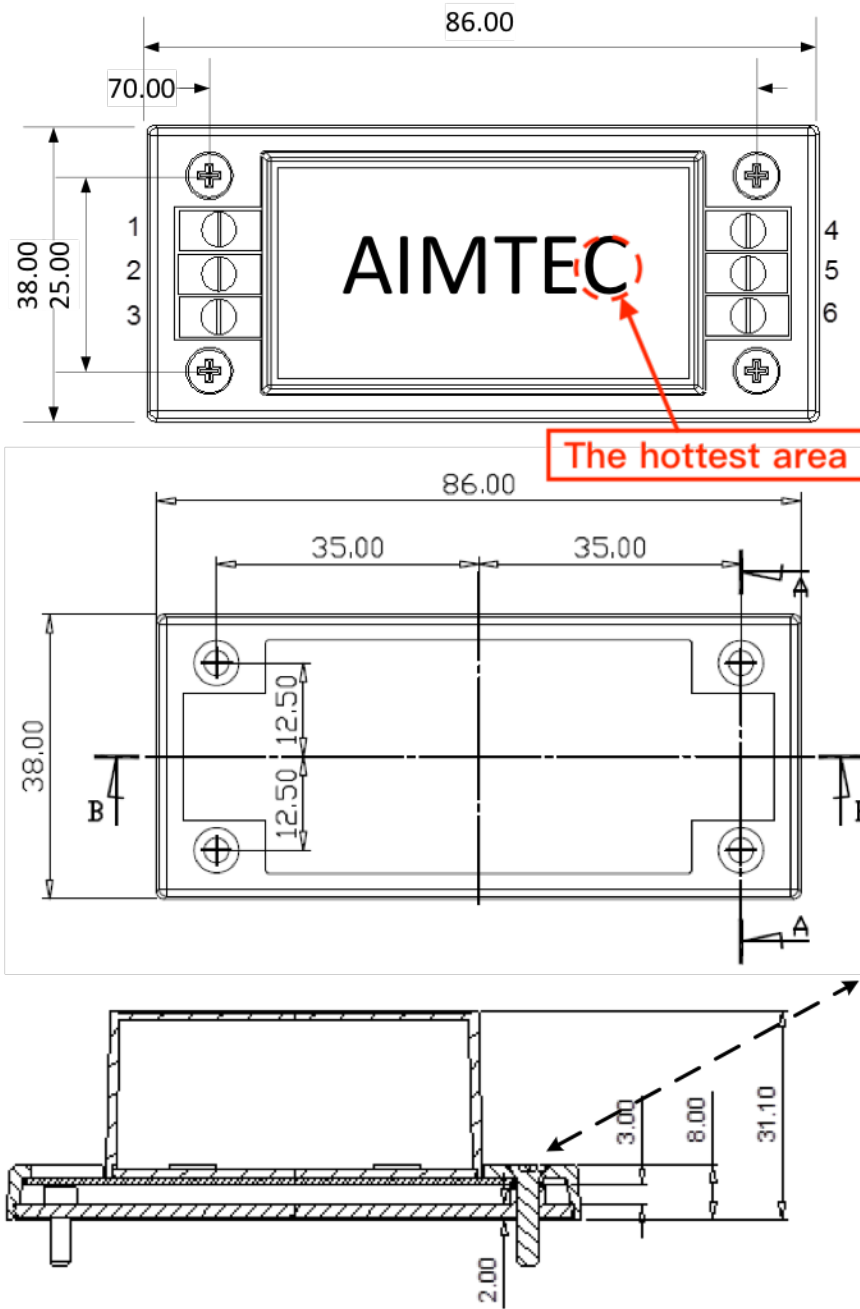
Pin Out Specification ST Version
